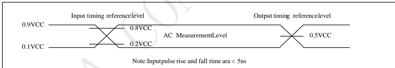
Figure 5-2 Input Test Waveforms and Measurement Level
